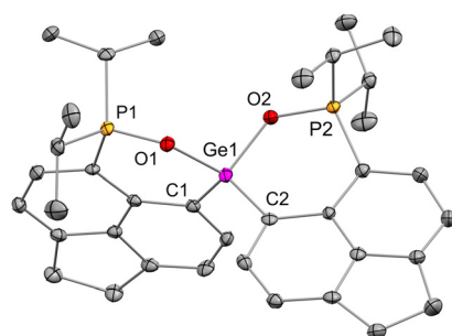
Fig. 2 Molecular structure of 1 IP PO in the solid state (thermal ellipsoid 35%, H atoms, triflate counter anions and solvent molecules are omitted for clarity). Selected bond lengths [Å] Ge1–O1 = 1.803(2), Ge1–C1 = 1.895(3), P1–O1 = 1.575(2), Ge1–O2 = 1.797(3), Ge1–C2 = 1.891(3), P2–O2 = 1.570(2); selected bond angles [°]: O1–Ge1–C1 = 103.9(1), O2–Ge1–C2 = 104.1(1), O1–Ge1–O2 = 105.1(1), C1–Ge1–C2 = 121.9(1).
