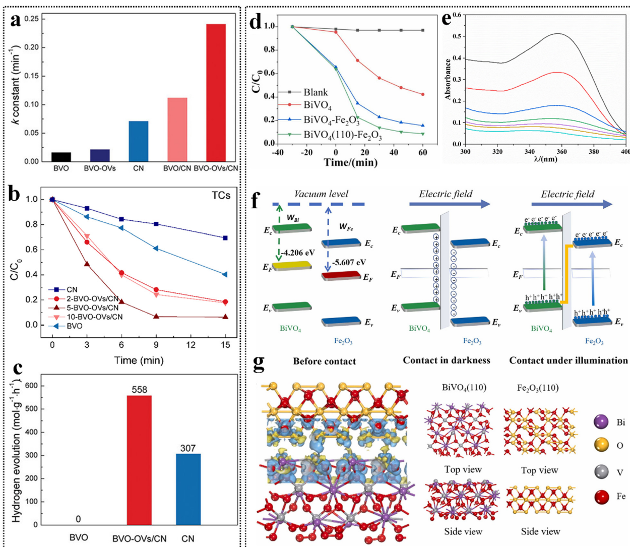
Fig. 8 (a) Corresponding first-order kinetic k constant of BVO, BVO-OVs, CN, BVO/CN, and BVO-OVs/CN. (b) Photodegradation on TC pollutant of BVO, CN and BVO-OVs/CN with different BVO-OVs/CN and CN ratios. (c) Comparison of photocatalytic hydrogen evolution rate. Reproduced from ref. 155 with permission from Wiley, copyright 2024. (d) Photocatalytic degradation of tetracycline by different samples. (e) Curve of absorbance with tetracycline concentration during the degradation of tetracycline by BiVO 4 (110)-Fe 2 O 3 . (f) Schematic diagram of the formation process of the electron transfer mechanism of Z-scheme heterojunctions. (g) Charge density difference diagram of BiVO 4 (110)-Fe 2 O 3 . Reproduced from ref. 156 with permission from Elsevier, copyright 2023.
