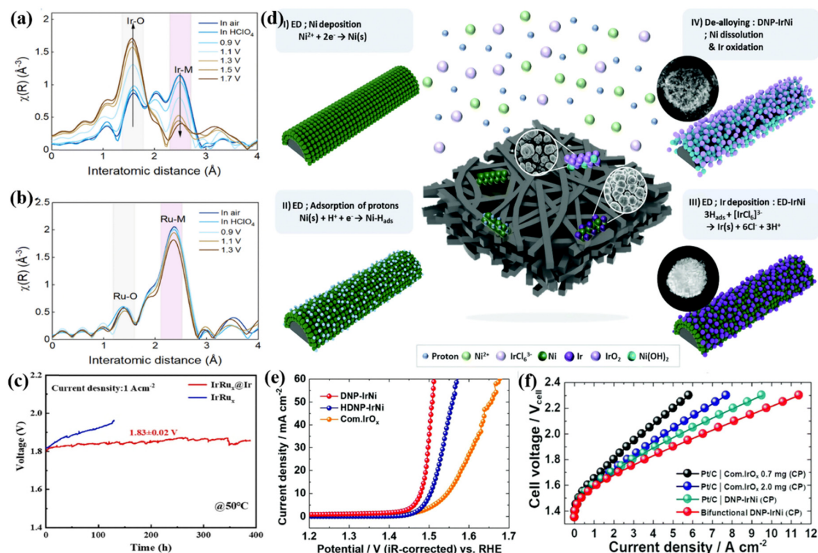
Fig. 3 (a) Ir and (b) Ru of in situ Fourier transformed extended X-ray absorption fine structure (EXAFS) spectra for \text{IrRu}_4/\text{TiC} . Reproduced with permission from ref. 103. Copyright 2022, The Royal Society of Chemistry. (c) Stability test of PEMWE with \text{IrRu}_x@\text{Ir} and \text{IrRu}_x catalysts as the anode at 1 \text{ A cm}^{-2} , respectively. Reproduced with permission from ref. 115. Copyright 2022, Elsevier B.V. (d) Schematic illustration of the experimental process for 3D DNP-IrNi. (e) OER polarization curves of DNP-IrNi and HDNP-IrNi. (f) Single PEMWE cell polarization curves combined with DNP-IrNi catalyst and carbon paper. Reproduced with permission from ref. 108. Copyright 2022, The Royal Society of Chemistry.
