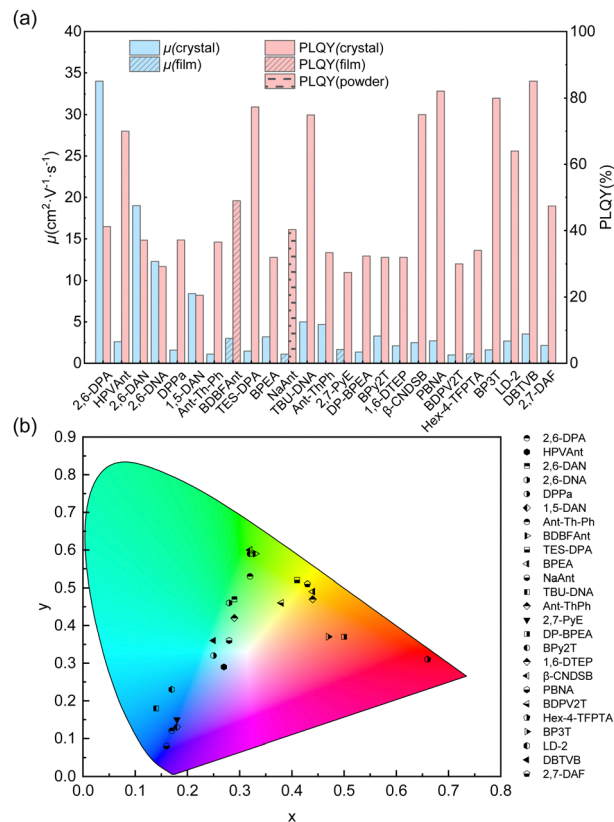
Fig. 2 Summary of the charge carrier mobility ( \mu ), PLQY (a) and emission colours (b) of high performance ( \mu_{\text{max}} > 1 \text{ cm}^2 \text{ V}^{-1} \text{ s}^{-1} , PLQY > 20%) small-molecule organic fluorescent semiconductors.
