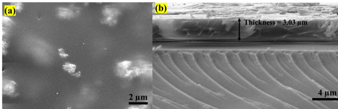
Fig. 7 (a) FESEM image of a PMMA-NBF film and (b) cross-sectional FE-SEM image of a PMMA-NBF thin film.
