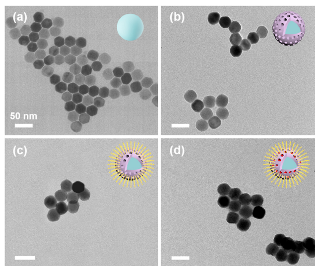
Fig. 1 Transmission electron microscopy (TEM) images of (a) \text{NaYF}_4:\text{Yb},\text{Er} (named UCNP s), (b) UCNP s@mPDA (UP), (c) UCNP s@mPDA@L-Arg (UPL), and (d) UCNP s@mPDA/ICG@L-Arg (UPIL). Scale bar: 50 nm.
