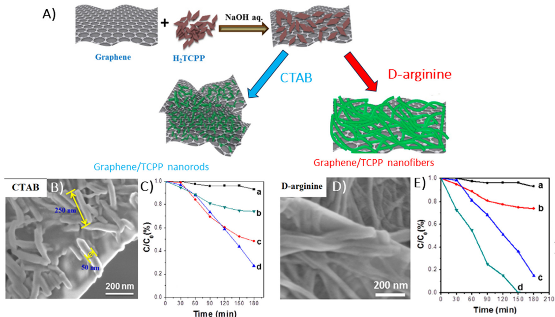
Fig. 26 (A) Diagram depicting the self-assembly of porphyrin aggregates on GNP mediated by arginine and CTAB, (B) SEM image showing porphyrin nanorods on GNPs, (C) photocatalytic efficacy of GNP/TCPP assemblies obtained with the assistance of CTAB in degrading RhB: (a) control without catalyst, (b) GNPs, (c) free standing TCPP nanorods, and (d) GNP-supported TCPP nanorods, (D) SEM image of porphyrin nanofibers on GNPs, and (E) photocatalytic performance of GNP/TCPP assemblies obtained with the assistance of D-arginine during RhB degradation: (a) control without catalyst, (b) GNPs, (c) free-standing TCPP nanofibers, and (d) GNP/TCPP nanofibers. Adapted from ref. 143 and 144. Copyright 2017 Wiley-VCH Verlag GmbH & Co. KGaA, Weinheim.
