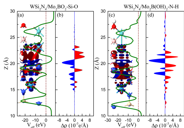
Fig. 5 Electrostatic potential and plane-averaged differential charge density \Delta\rho for \text{WSi}_2\text{N}_4/\text{Mo}_2\text{BO}_2 -Si-O (a) and (b) and \text{WSi}_2\text{N}_4/\text{Mo}_2\text{B}(\text{OH})_2 -N-H (c) and (d). The insets in panels (a) and (c) are the 3D isosurface of the electron charge density difference of \text{WSi}_2\text{N}_4/\text{Mo}_2\text{BO}_2 -Si-O and \text{WSi}_2\text{N}_4/\text{Mo}_2\text{B}(\text{OH})_2 -N-H, respectively.
