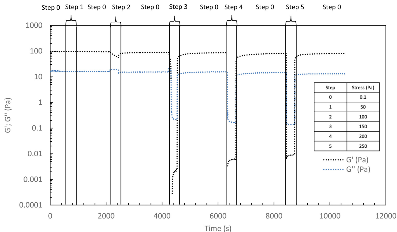
Fig. 9 Elastic and viscous moduli during different stress applications (ranging from 50 to 250 Pa) to the hydrogel (HA-PiPrOx-co-PBuOx-66/34-0.10, 15 \text{ g L}^{-1} in NaCl 0.15 M) at 37 °C (1 Hz) with a rest time (0.1 Pa, 1 Hz) between stresses.
