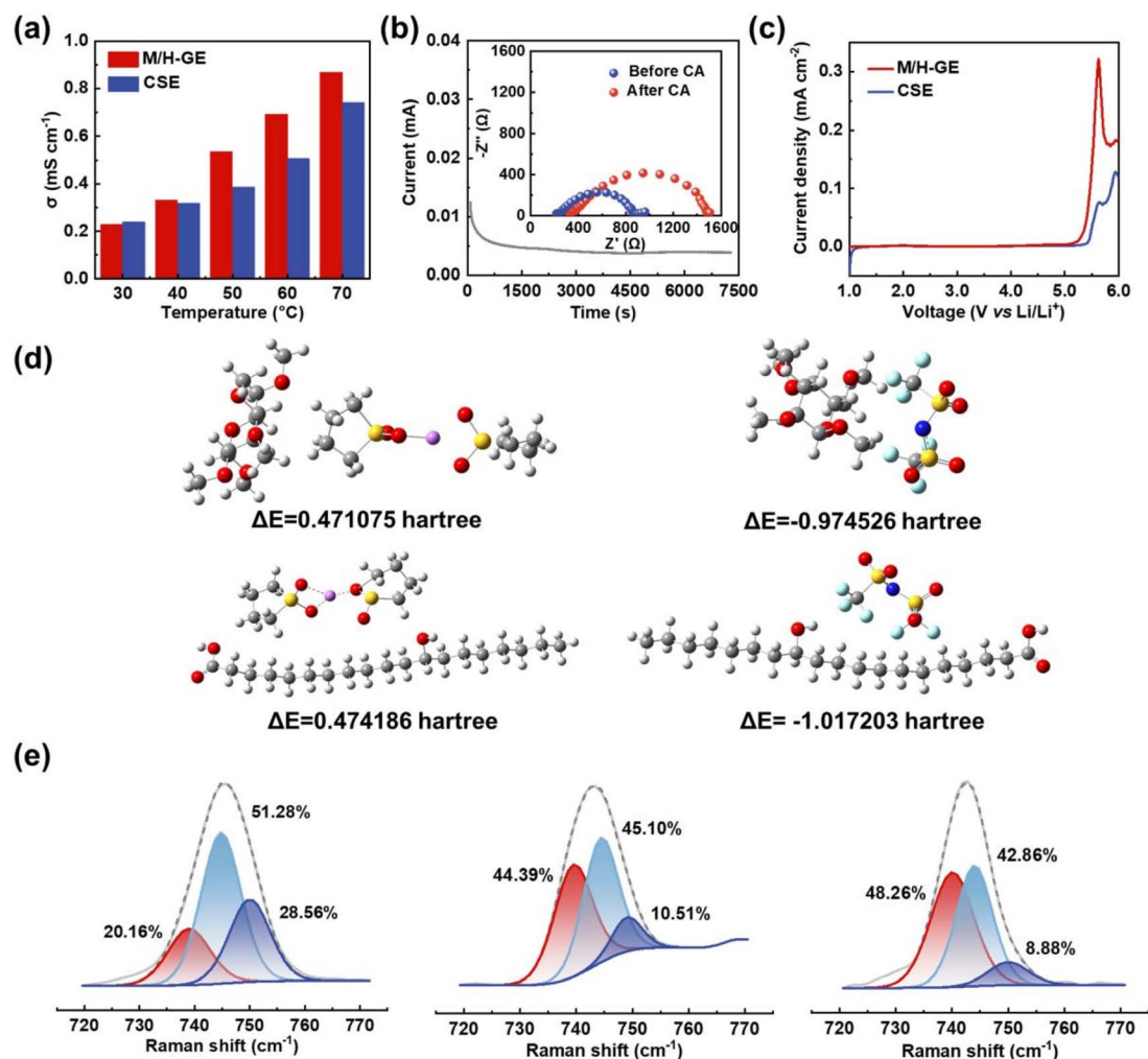
Fig. 5 \text{Li}^{+} conduction properties and mechanism of GEs: (a) EIS results of stainless steel symmetric cells using the M/H-GE membrane tested at 30–70 °C. (b) Direct current (DC) polarization of the Li||M/H-GE||Li cell at 10 mV (inset: EIS spectra before and after DC polarization). (c) LSV curves of the Li||M/H-GE||stainless steel cell and Li||CSE||stainless steel cell. (d) Simulated gelator- [\text{Li}(\text{SL})_2]^{+} complex cation interactions and gelator- \text{TFSI}^{-} interactions. (e) Raman spectra of CSE, H-GE, M/H-GE membrane.
