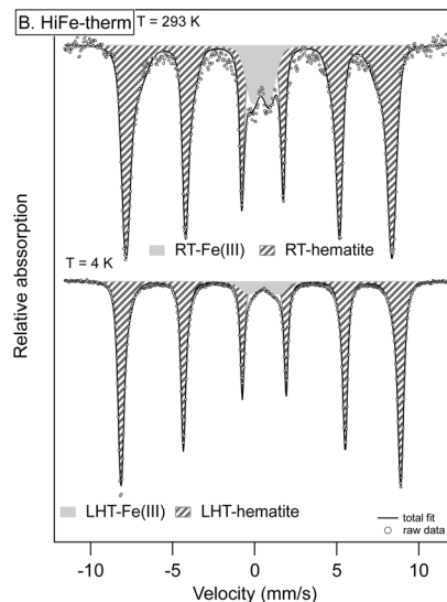
Fig. 9 Mössbauer spectra of HiFe clay as-received (A), after thermal treatment (B) and after mechanical treatment (C). Spectra were collected at room temperature (RT: 293 K) and at low temperature (LHT: 4 K). Hyperfine parameters of the Fe components used in the fit are listed in Table S5 in the ESI.†
