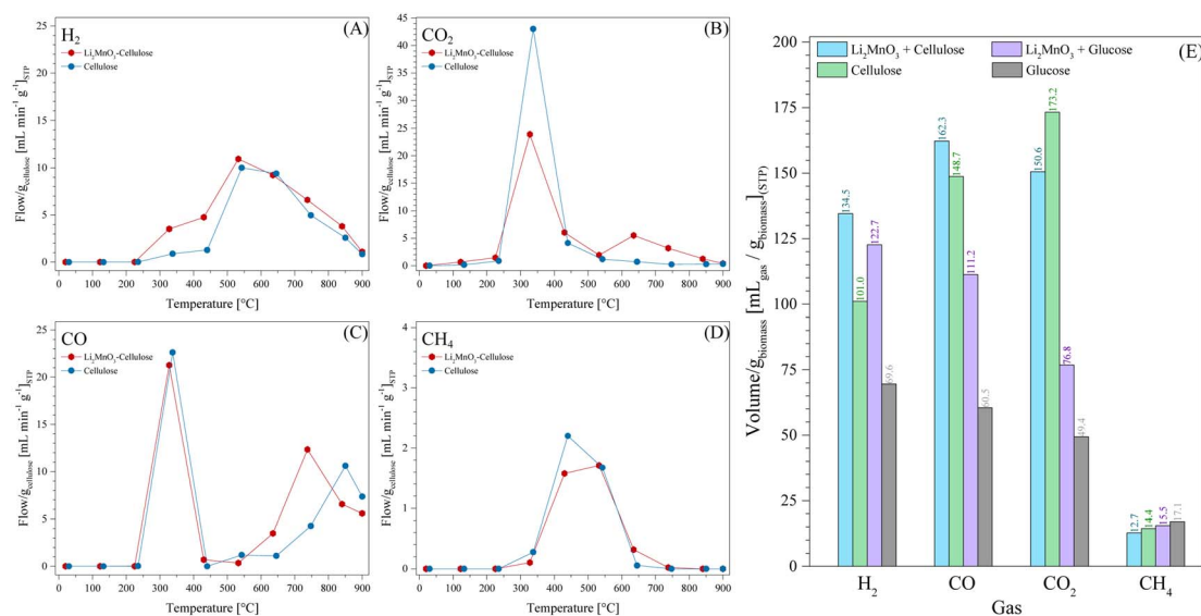
Fig. 10 Thermal evolution of the produced gases (H 2 (A), CO 2 (B), CO (C) and CH 4 (D)) for LMO-C and cellulose samples, from 30 °C to 900 °C in N 2 , using a heating rate of 30 °C min -1 , normalized per gram of cellulose. Total volume of the gaseous products (E) normalized per gram of biomass. Glucose and LMO-G 25-75 results are added for comparison.
