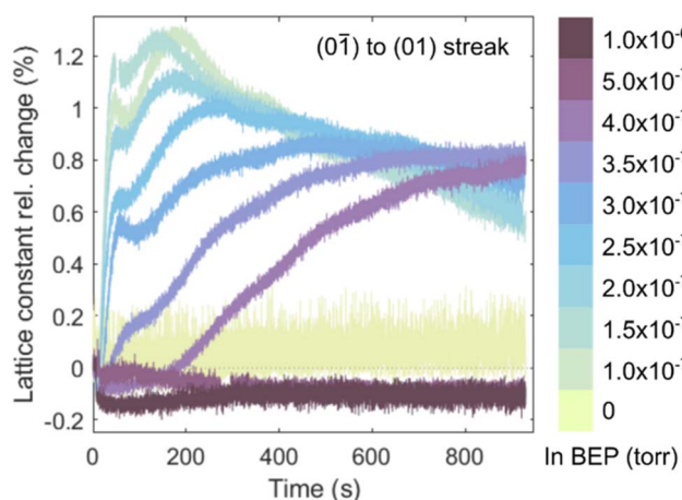
Fig. 5 Percentage change in d -spacing relative to the \text{Ga}_2\text{O}_3 c plane lattice constant vs. growth time for (0\bar{1}) to (01) streak spacing. All (\text{InGa})_2\text{O}_3 growths were performed at 723^\circ\text{C} and \text{Ga BEP} = 1.5 \times 10^{-7} torr. In BEP in torr is indicated by color bar and varies from zero to 1 \times 10^{-6} torr.
