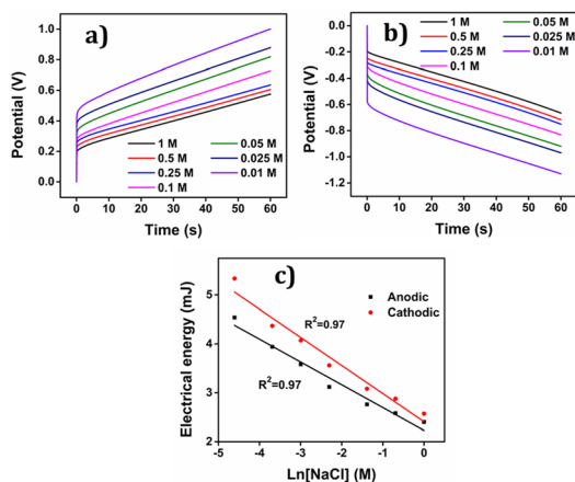
Fig. 17 Chronopotentiogram obtained from different concentrations of NaCl when (a) 0.05 mA and (b) -0.05 mA of current were applied to the PEDOT for 60 s. (c) Electrical energy ( U ) consumed by the film during the reaction as a logarithmic function of electrolyte concentration at room temperature.
