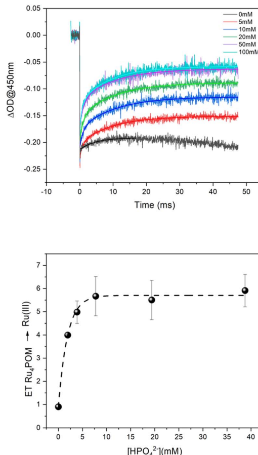
Fig. 2 (Top panel) Kinetic traces at 450 nm obtained by laser flash photolysis of 100 \mu\text{M} \text{Ru}(\text{bpy})_3\text{Cl}_2 , 5 mM \text{Na}_2\text{S}_2\text{O}_8 , 2.5 \mu\text{M} \text{Na}_{10}\text{Ru}_4\text{POM} , 0.1 M \text{Na}_2\text{SO}_4 in unbuffered water and in 5–100 mM phosphate buffer at pH 7.0. The solid lines indicate the biexponential fittings of the traces (monoexponential fitting in the trace in water). (Bottom panel) Plot of the number of \text{Ru}_4\text{POM} \rightarrow [\text{Ru}(\text{bpy})_3]^{3+} ET events in 50 ms vs. the concentration of \text{HPO}_4^{2-} (base of the buffer). The number of ET events is estimated from the experimental recovery of the bleach in the kinetic traces in the top panel. The error bars are given as semi-dispersion of two separate experiments.
