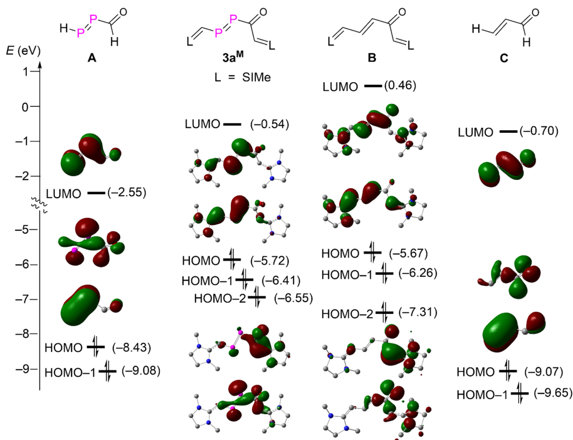
Fig. 4 Energy diagram for the frontier Kohn-Sham orbitals (isovalue = 0.04) of compound 3\mathbf{a}^{\text{M}} and A–C.
