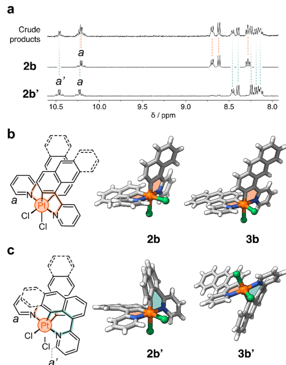
Fig. 3 (a) Partial 1 H NMR spectra (400 MHz, DCM- d 2 ) of the reaction crude product obtained from the oxidation of 2a. (b) Chemical structure and solid-state structures of complexes (b) 2b and 3b, and (c) 2b' and 3b'. Panels (b) and (c) contain the proton assignment of resonances a and a '.
