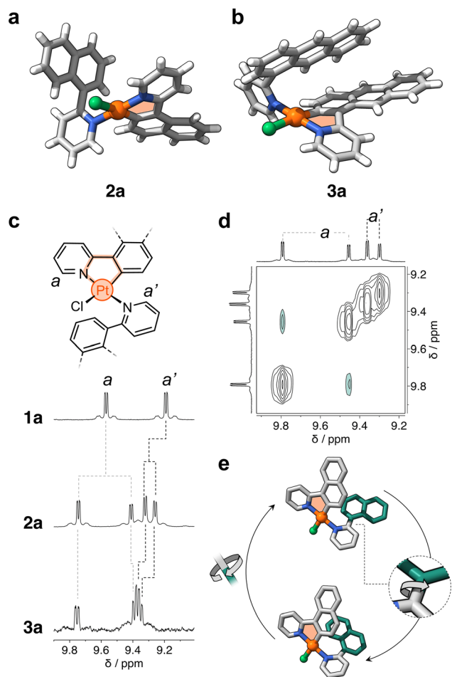
Fig. 2 Solid-state molecular structures of complexes (a) 2a and (b) 3a. (c) Representative chemical structure of complexes 1a, 2a, and 3a. Partial 1 H NMR spectra (400 MHz, DCM- d 2 ) of such complexes is shown in this panel. (d) Partial EXSY NMR spectrum (600 MHz, DCM- d 2 ) of complex 2a showing cross peaks between the signals of two atropisomers. (e) Proposed rotational dynamics observed in complex 2a in solution. The structures correspond to the two DFT-computed isomers. Hydrogen atoms omitted for clarity. The cyclometalated and free-rotating naphthalenyl moieties are colored grey and green, respectively.
