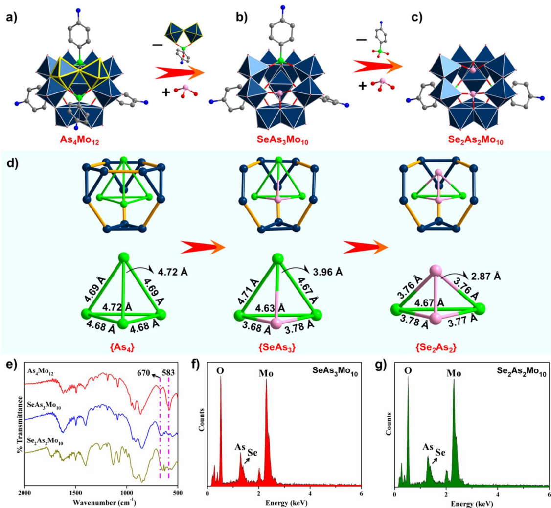
Fig. 1 (a)–(c) Structural evolution from the plenary \text{As}_4\text{Mo}_{12} species to the di-lacunary species, \text{SeAs}_3\text{Mo}_{10} and \text{Se}_2\text{As}_2\text{Mo}_{10} . Color code: {MoO 6 }, dark blue octahedra; As, green; Se, pink; C, gray; N, blue; O, red. (d) Structural symmetry of \text{As}_4\text{Mo}_{12} and the as-made polyanions. (e) FT-IR spectra of \text{As}_4\text{Mo}_{12} , \text{SeAs}_3\text{Mo}_{10} and \text{Se}_2\text{As}_2\text{Mo}_{10} . (f) and (g) EDX analysis of \text{SeAs}_3\text{Mo}_{10} and \text{Se}_2\text{As}_2\text{Mo}_{10} .
