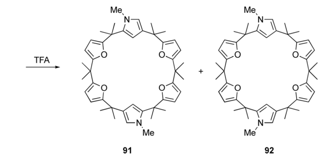
Scheme 14 Strain-induced ring expansion of calix[3]pyrrole analogues.
