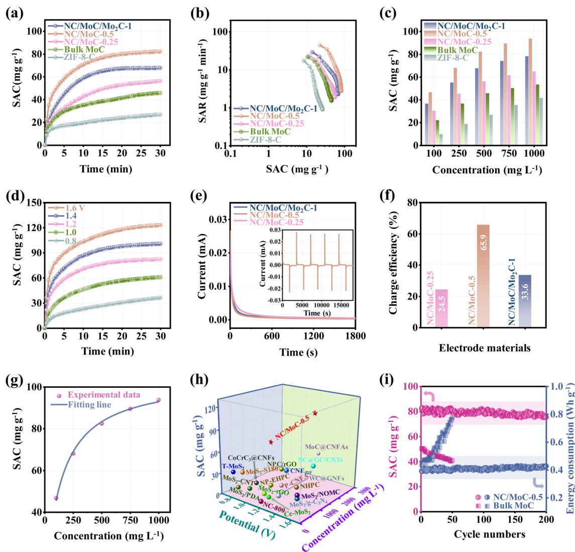
Fig. 4 (a) Dynamic SAC versus deionization time plots, and (b) corresponding CDI Ragone plots of the three NC/MoC-x, bulk MoC, and ZIF-8-C in 500 mg L -1 NaCl solution at 1.2 V. (c) SAC values at different NaCl concentrations from 100 to 1000 mg L -1 for the three NC/MoC-x, bulk MoC, and ZIF-8-C (applied voltage: 1.2 V). (d) Dynamic SAC versus deionization time plots of NC/MoC-0.5 with an initial concentration of 500 mg L -1 using different voltage from 0.8 to 1.6 V. (e) Current response curves of the three NC/MoC-x, and the corresponding current variation of NC/MoC-0.5 during the desalination/regeneration cycle (inset). (f) The calculated charge efficiencies of the three NC/MoC-x. (g) The fitted isotherm adsorption curves of the Langmuir model (applied voltage: 1.2 V; NaCl concentration: from 100 to 1000 mg L -1 ). (h) Comparison of CDI performance between NC/MoC-0.5 and some reported transition metal carbides/dichalcogenides or MOF-derived carbons. (i) The recycling performance of bulk MoC and NC/MoC-0.5, along with their corresponding energy consumption changes over 200 cycles (applied voltage: 1.2 V; NaCl concentration: 500 mg L -1 ).
