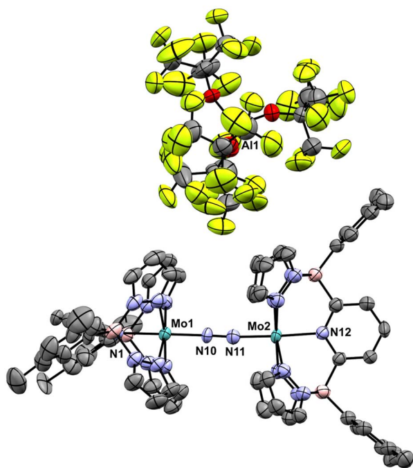
Fig. 5 Molecular structure of [\text{3-Xyl}]^{+} . Thermal ellipsoids are shown at the 50% probability level and all H atoms are omitted for clarity. Selected bond distances (Å): Mo(1)–N(1), 2.167(5); Mo(1)–N(10), 1.885(5); Mo(2)–N(12), 2.080(5); Mo(2)–N(11), 1.916(6); N(10)–N(11), 1.162(7) cf. N–N distance in free \text{N}_2 of 1.098. Selected bond angles ( ^{\circ} ): N(1)–Mo(1)–N(10), 176.6(2); Mo(1)–N(10)–N(11), 173.8(5); N(10)–N(11)–Mo(2), 175.5(4); N(11)–Mo(2)–N(12), 177.2(3).
