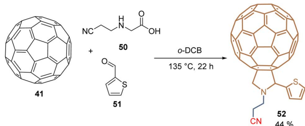
Scheme 3 Prato reaction for the synthesis of fulleropyrrolidine 52 substituted with the thiophene moiety.
