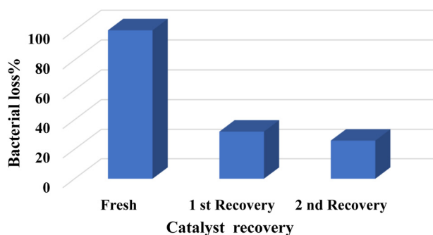
Fig. 6 Effect of powder catalyst recovery and reuse on S. aureus loss. Experiment conducted using fresh anatase TiO_2 (0.1 g), first recovered and second recovered catalyst. Fresh bacterial solution (50 mL, 1 \times 10^6 CFU mL -1 ) is used in each catalyst, with pH 6.2, for 1 h at 25 \pm 2 °C under a radiation intensity of 0.136 W cm -2 . Error is 10%.
