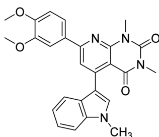
7-(3,4-Dimethoxyphenyl)-1,3-dimethyl-5-(1-methyl-1H-indol-3-yl)pyrido[2,3-d]pyrimidine-2,4(1H,3H)-dione
