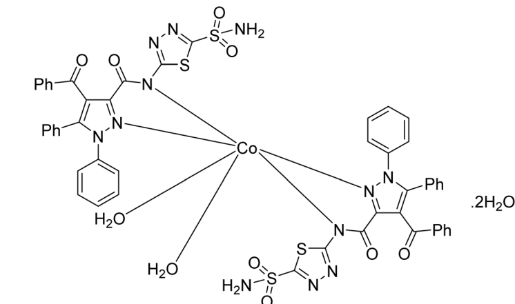
(Diaquabis(4-benzoyl-1,5-diphenyl-N-(5-sulfamoyl-1,3,4-thiadiazol-2-yl)-1H-pyrazole-3-carboxamide)cobalt(II) dihydrate
