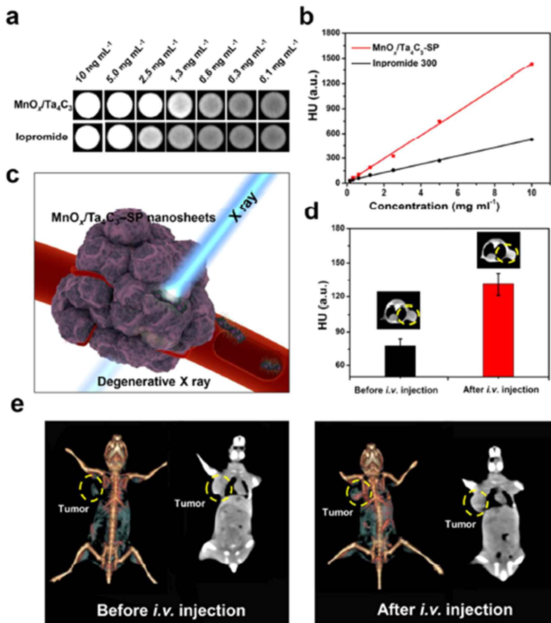
Fig. 15 (a) In vitro CT images and (b) CT contrasts of \text{MnO}_x/\text{Ta}_4\text{C}_3\text{-SP} composite nanosheet solutions and iopromide solutions at varied concentrations (0.1, 0.3, 0.6, 1.3, 2.5, 5.0, and 10 \text{mg mL}^{-1} with respect to Ta and I, respectively). (c) Schematic of in vivo CT imaging by using \text{MnO}_x/\text{Ta}_4\text{C}_3\text{-SP} composite nanosheets as the contrast agents. (d) In vivo CT contrasts of tumor tissue before and after i.v. administration of \text{MnO}_x/\text{Ta}_4\text{C}_3\text{-SP} composite nanosheets. (e) In vivo 3D reconstruction CT images (left) and contrast images (right) of mice before and after i.v. administration of \text{MnO}_x/\text{Ta}_4\text{C}_3\text{-SP} composite nanosheets (20 \text{mg kg}^{-1} , 100 \mu\text{L} ) for 2 h (Reproduced from ref. 109 with permission from American Chemical Society copyright [2024]).
