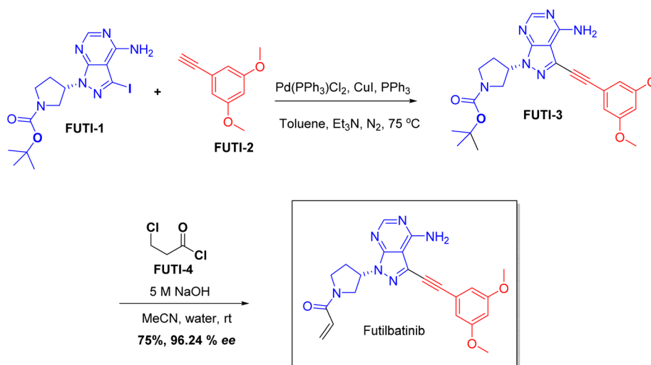
Scheme 4 Synthesis of futibatatinib.
