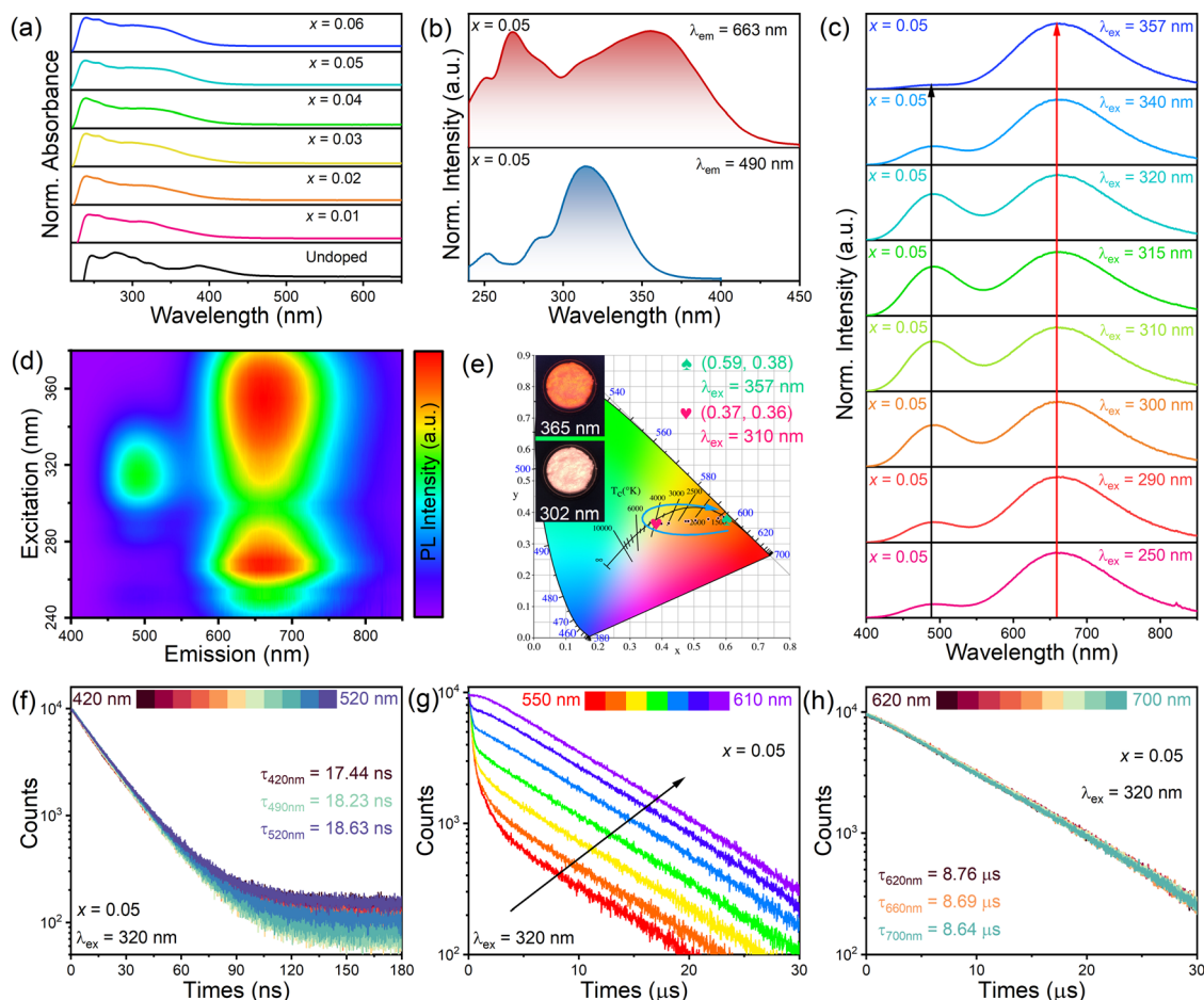
Fig. 2 (a) Absorption spectra of the (\text{TMA})_2\text{HfCl}_6:\text{xSb}^{3+} ( x = 0-0.06 ). (b) PL excitation (PLE) of 663 and 490 nm emission in (\text{TMA})_2\text{HfCl}_6:0.05 \text{ Sb}^{3+} crystals. (c) PL spectra of (\text{TMA})_2\text{HfCl}_6:\text{Sb}^{3+} under different excitation wavelengths varying from 250 to 357 nm. (d) Contour plot of the excitation-dependent photoluminescence of the (\text{TMA})_2\text{HfCl}_6:0.05 \text{ Sb}^{3+} crystals. (e) The corresponding CIE color coordinates of the (\text{TMA})_2\text{HfCl}_6:0.05 \text{ Sb}^{3+} samples under different excitation wavelengths. (the inset are the photos of the as-prepared samples under different UV lamp). PL decay curves of (\text{TMA})_2\text{HfCl}_6:0.05 \text{ Sb}^{3+} in emission wavelength range of (f) 420–450 nm, (g) 550–610 nm, and (h) 620–700 nm excited by 320 nm.
