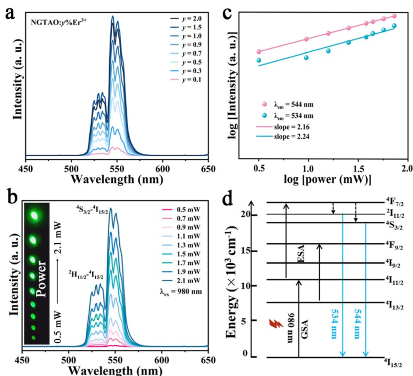
Fig. 4 Dependence of the UCL spectra on the 980 nm laser power density. (a) PL spectra of NGTAO:y%Er 3+ ( 0.1 \leq y \leq 2.0 ) under 379 nm excitation. (b) UCL spectra of NGTAO:1.0%Er 3+ at different pump powers and (c) double logarithmic plots of excitation power versus UCL intensity of Er 3+ at 534 nm and 544 nm for NGTAO:1.0%Er 3+ . (d) Energy level diagram and corresponding possible UC processes of NGTAO:Er 3+ .
