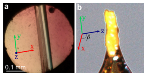
Fig. 3 Single crystal of 3 : (a) as grown in the DAC and (b) after being recovered to ambient conditions and transforming to 1 , mounted on a nylon loop. Crystal axes are indicated.
