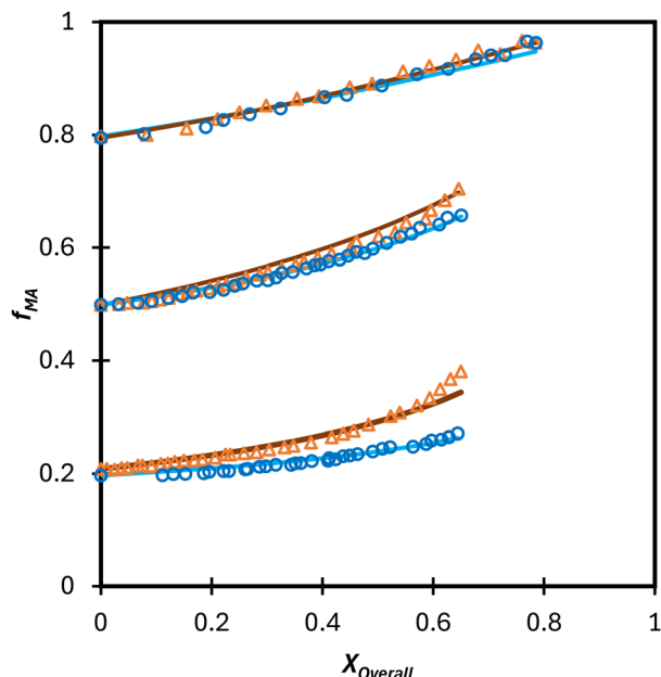
Fig. 5 Drift in MA comonomer composition ( f_{MA} ) with overall monomer conversion for the copolymerization of MA/MAA in DMSO- d_6 with w_{mon,0} = 0.5 ( \Delta ) and 0.1 ( \circ ). Lines are simulated using the best-fit reactivity ratio estimated from corresponding data set.
