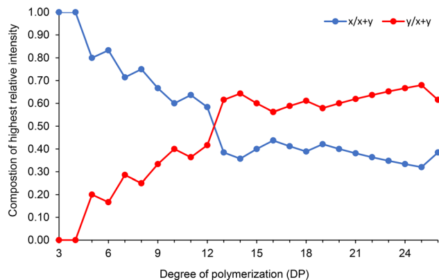
Fig. 8 Variation of the composition ( x , y ) in \text{P}[(\text{CL}^{\text{nBu}})_x\text{-co-(CL}^{\text{Me}})_y] copolymers as a function of the degree of polymerization (DP). The composition was calculated from the most intense m/z signal for a defined DP, from MALDI-ToF MS of \text{P}[(\text{CL}^{\text{nBu}})_x\text{-co-(CL}^{\text{Me}})_y] copolymers prepared by the ROCOP of a 1 : 1 mixture of ( R )- \text{CL}^{\text{nBu}} and ( S )- \text{CL}^{\text{Me}} with the 1a /BnOH catalytic system, over 35 min (Table 1, entry 1).
