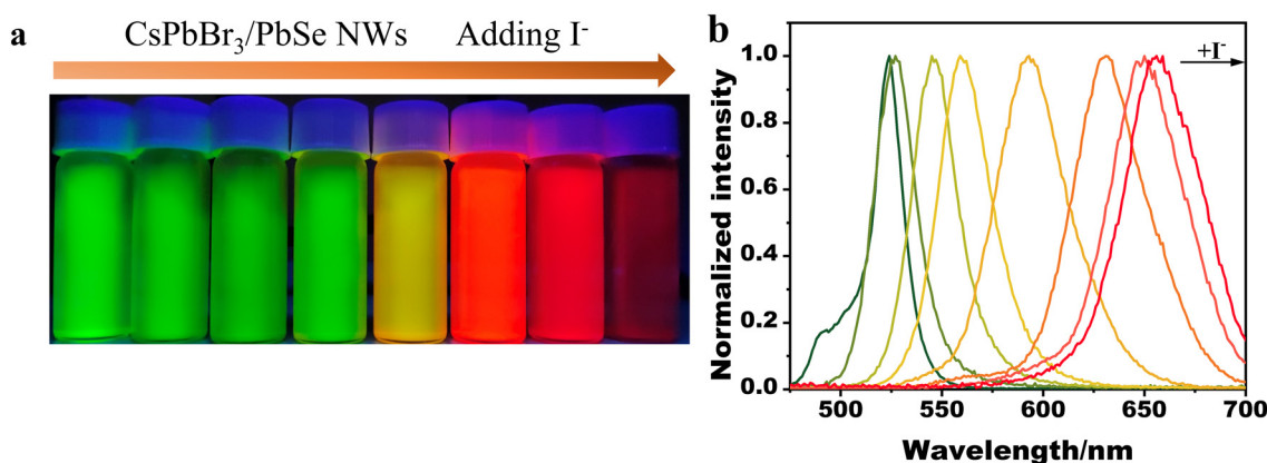
Fig. 4 (a) Photograph of colloidal CsPbBr 3 /PbSe NWs reacting with different concentrations of I − ions under a 365 nm UV lamp; (b) corresponding photoluminescence spectra of colloidal CsPbBr 3 /PbSe perovskite NWs.
