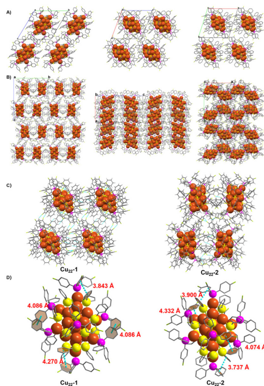
Fig. 3 Views of the assembled packing of (A) Cu 22 -1 and (B) Cu 22 -2 viewed along the a , b and c axes. (C) The intermolecular forces of C–F...H–C in the isomeric Cu 22 -1 and Cu 22 -2. (D) The intramolecular forces of \pi ... \pi in the isomeric Cu 22 -1 and Cu 22 -2. Cu = brown, Se = yellow, P = purple, F = chartreuse, C = gray. For clarity, H atoms are omitted.
