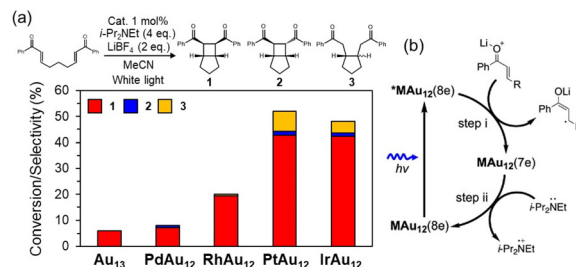
Fig. 6 (a) Comparison of the photoredox catalytic properties of \text{MAu}_{12}(\text{dppe})_5\text{Cl}_2 ( \text{MAu}_{12} ; M = Au, Pd, Pt, Rh, or Ir). (b) Proposed reaction mechanism for \text{MAu}_{12} , a so-called oxidative quenching cycle. Reproduced from ref. 58 with permission from Wiley-VCH, Copyright 2023.
