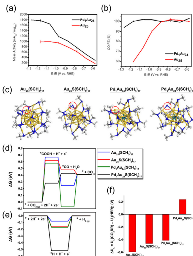
Fig. 4 (a) \text{CO} mass activity and (b) faradaic efficiency for \text{CO} in the \text{CO}_2\text{RR} over \text{Au}_{25}(\text{PET})_{18}/\text{C} and \text{PdAu}_{24}(\text{PET})_{18}/\text{C} . (c) DFT-optimized structures of \text{MAu}_{24}(\text{SCH}_3)_{18} and \text{MAu}_{24}\text{S}(\text{SCH}_3)_{17} ( \text{M} = \text{Pd}, \text{Au} ). Proposed active sites are circled in red. Colour code: Au, yellow; Pd, turquoise; S, blue; C, gray; H, white. Gibbs free energy diagrams for the (d) \text{CO}_2\text{RR} and (e) HER at U = 0 V vs. RHE. (f) Difference in the predicted limiting potentials for the \text{CO}_2\text{RR} and HER. Reproduced from ref. 51 with permission from the American Chemical Society, Copyright 2020.
