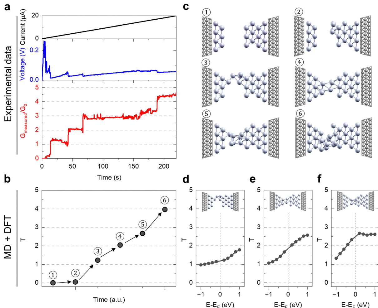
Fig. 3 Rewiring through quantum conductance effects. (a) Quantum conductance effects in a current sweep induced NW rewiring. A current sweep in the range 0–20 μA was applied to the NW device (sweep rate of \sim 90 \text{ nA s}^{-1} ) while measuring the voltage drop across its electrodes, allowing the monitoring of the device conductance G_{\text{measured}} . (b) Evolution of the transmission coefficient during the rewiring process computed by DFT simulations on the structures depicted in (c). Dependence of the transmission coefficient on the applied voltage (d), (e) and (f) respectively for structure 3, 4 and 5 of Panel c.
