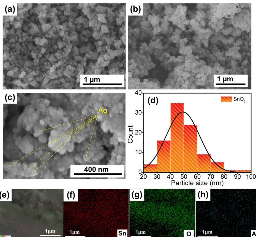
Fig. 2 SEM images of (a) SnO 2 and (b and c) Ag TNPs/SnO 2 ; (d) particle size distribution histogram of SnO 2 in the Ag TNPs/SnO 2 sample; (e–h) SEM-EDS elemental mapping of Ag TNPs/SnO 2 .
