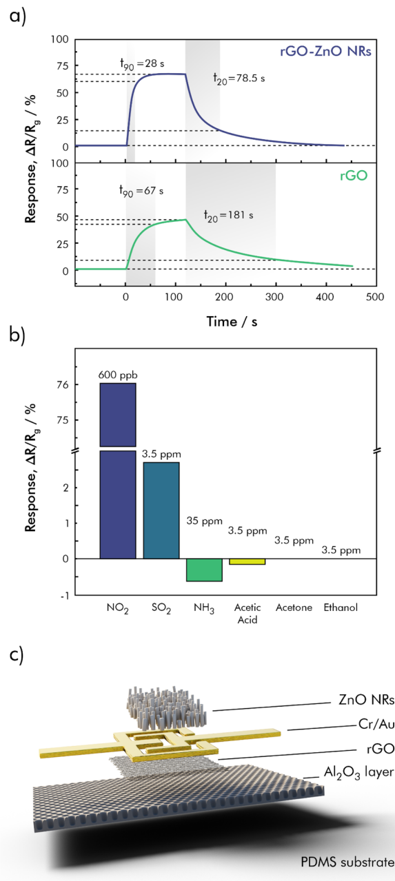
Fig. 9 (a) Dynamic response recovery curves from rGO and the rGO-ZnO NR towards NO 2 at a concentration of 400 ppb, (b) selectivity test using NO 2 (600 ppb), SO 2 (3.5 ppm), NH 3 (35 ppm), acetic acid (3.5 ppm), acetone (3.5 ppm), and ethanol (3.5 ppm); (c) sensor geometry of the stacked rGO-ZnO NR hybrid sensor; redrawn and adapted, with permission from ref. 130.
