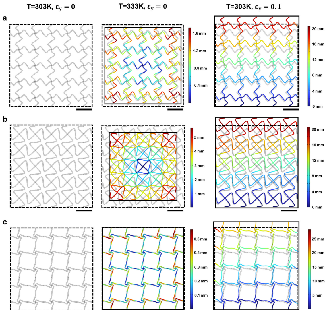
Fig. 3 Numerical simulation results of the BPCM for PR and CTE, scale factor = 4.5: (a) \text{CTE} = -237.356 \text{ ppm K}^{-1} , \text{PR} = -0.1327 , (b) \text{CTE} = -844.864 \text{ ppm K}^{-1} , \text{PR} = -0.0989 and (c) \text{CTE} = -31.5737 \text{ ppm K}^{-1} , \text{PR} = -0.5655 (all the scale bars are 40 mm).
