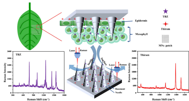
Fig. 5 A schematic representation of the pesticide residue in agricultural products using MNs. The image was reproduced with permission 86 from ACS, copyright@2023.
