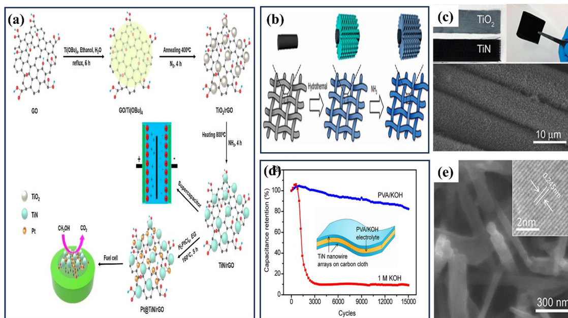
Fig. 12 (a) The production processes of the \text{Pt}@\text{TiN}/\text{rGO} ternary hybrid and the \text{TiN}/\text{rGO} composite (reproduced from ref. 157 with permission); (b) schematic of a two-step growth method for generating \text{TiN} nanowires (NWs) on carbon cloth; (c) images of carbon cloth coated with \text{TiO}_2 and \text{TiN} nanoparticles, as well as a SEM image showcasing \text{TiN} NWs growth on carbon fabric; (d) comparison of \text{H-TiN} NPs and \text{TiN} NTs electrode electrochemical performances; (e) an enlarged SEM perspective of a single carbon fiber embellished with \text{TiN} nanowires (reproduced from ref. 158 with permission).
