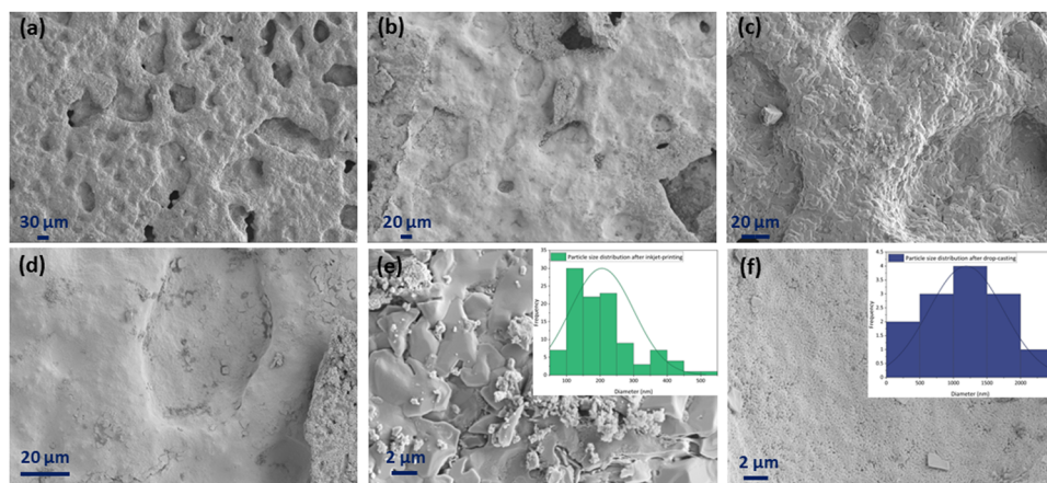
Fig. 10 Surface SEM images of (a), (c) and (e) 100-layer and (b), (d) and (f) drop-cast porous NLK–GDC symmetric cells in 185\times (a and b), 687\times (c and d), and 4.15\text{k}\times (e and f) magnifications. The insets of (e) and (f) figures are the particle size distributions of \text{CuFe}_2\text{O}_4 particles on the surface of the inkjet-printed and drop-cast samples, respectively, analyzed using ImageJ software.
