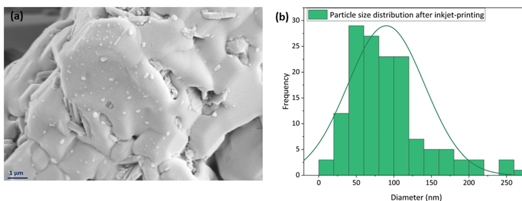
Fig. 11 (a) Surface SEM image with a high magnification of 8.66\text{k}\times from the 100-layer inkjet-printed sample and (b) \text{CuFe}_2\text{O}_4 nanoparticle size distribution on its surface, analyzed using ImageJ software.
