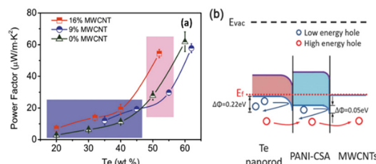
Fig. 4 (a) Comparison of TE properties and (b) interfacial energy filtering effects. [Reproduced from ref. 31, with permission from Wiley VCH, Copyright 2018.]
