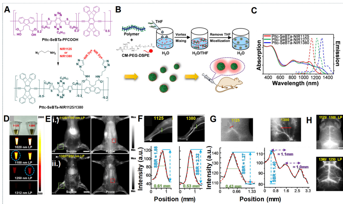
Fig. 13 (A) Synthesis scheme for PtSeB-Ta-NIR1125/1380 semiconducting polymers. (B) Schematic for the preparation of PtSeB-Ta-NIR1125/1380 Pdots. (C) Absorption and emission spectra represented as solid and dashed lines, respectively, corresponding to PtSeB-Ta-NIR1125, PtSeB-Ta-NIR1380 and PtSeB-Ta-NIR1270 Pdots in water shown as red, blue and green lines, respectively. (D) Images shown under ambient light (first row) of PtSeB-Ta-NIR1125 and PtSeB-Ta-NIR1380 Pdots (left and right) with LPFs at 1020 nm, 1100 nm, 1250 nm, and 1312 nm (bottom rows) under 808 nm laser excitation. (E) Whole-body imaging of mice post intravenous administration of PtSeB-Ta-NIR1125/1380 Pdots imaged with different LPFs with wavelengths of 1100 nm and 1250 nm, respectively, in supine and prone positions shown in left and right images. (F) Enlarged images of mouse hind limb vasculature highlighted in the green squares of (E, i) and (E, ii) (top and bottom row, left), with green lines showing their respective cross-sectional intensity profiles in (F) for PtSeB-Ta-NIR1125 (left)/1380 (right). (G) Expanded view of the area in the red squares marked on the spinal cord of (E, i) (top row, right) and (E, ii) (bottom row, right), with the red lines showing their respective cross-sectional intensity profiles for PtSeB-Ta-NIR1125/1380 Pdots (right). (H) Wild-type C57BL/6 mouse brain vasculature NIR-II fluorescence imaging post-intravenous injection of PtSeB-Ta-NIR1125/1380 Pdots displayed in top and bottom images using 1100 nm and 1250 nm LPF. Adapted with permission from ref. 49, from John Wiley and Sons, copyright © 2020.
