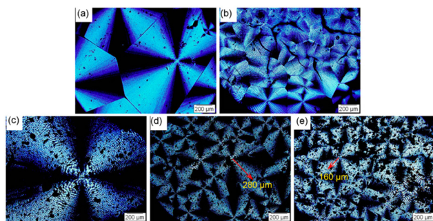
Fig. 24 Micrographs of (a) PHBV, (b) crosslinked PHBV, (c) PHBV-lignin blend, (d) PHBV-1-lignin with 1% DCP, and (e) PHBV-2-lignin with 1% DCP crystallized at 90 °C. Scale bar: 200 \mu\text{m} . Reproduced from ref. 155 with permission from American Chemical Society, copyright 2016.
