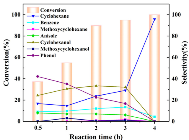
Fig. 6 Results of varying the reaction time on the HDO of guaiacol. Conditions: 0.1 g guaiacol 0.05 g Ni_2Mo_3N/C 20 mL octane 260 °C 1 MPa H_2 4 h.
