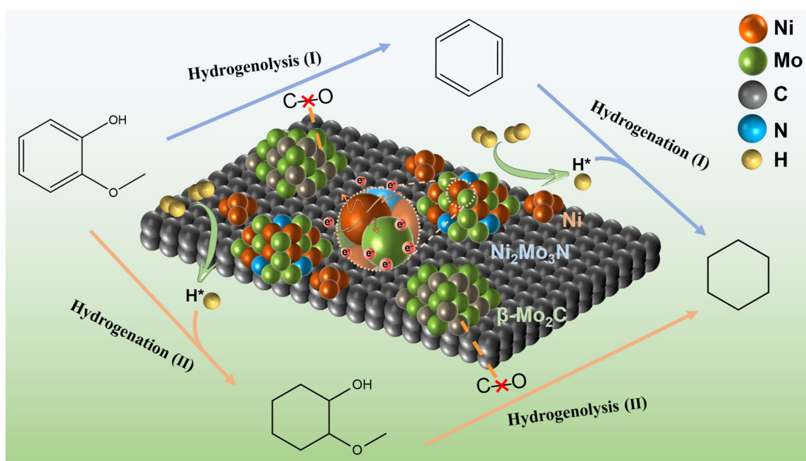
Fig. 7 Schematic illustration showing the catalytic role of the multiple active components in the catalysts and the possible HDO pathways of guaiacol over Ni_2Mo_3N/C catalyst.
