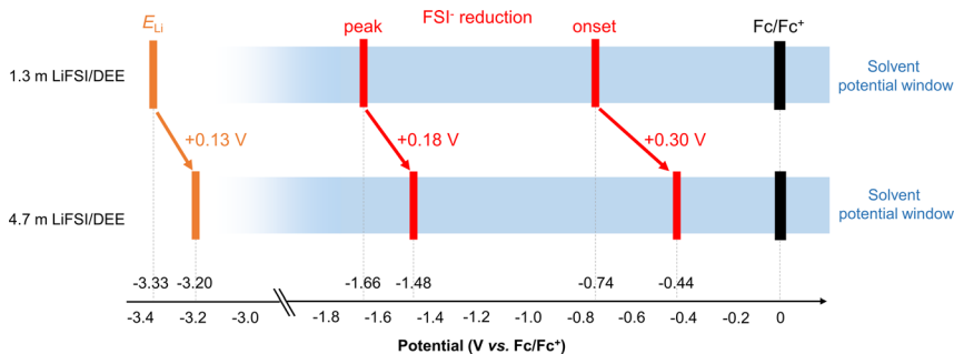
Fig. 6 Potential diagram of dilute (1.3 m) and concentrated (4.7 m) LiFSI/DEE that highlights the upward shift of E_{\text{Li}} and \text{FSI}^- reduction potential.
