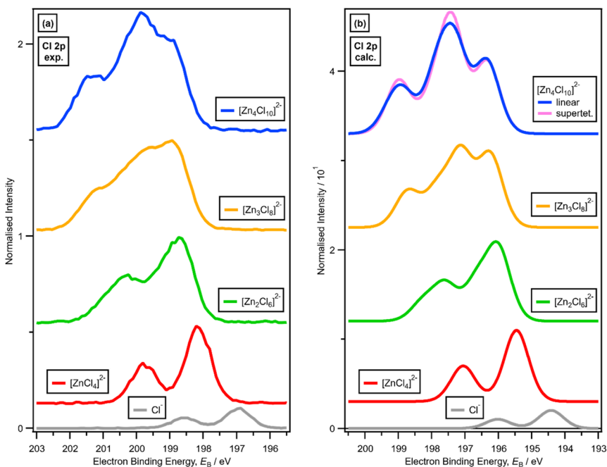
Fig. 6 (a) Experimental core Cl 2p XPS (going from bottom to top) for x = 0.00 [\text{C}_8\text{C}_{11}\text{Im}]\text{Cl} , x = 0.33 [\text{C}_8\text{C}_{11}\text{Im}]_2[\text{ZnCl}_4] , x = 0.50 [\text{C}_8\text{C}_{11}\text{Im}]_2[\text{Zn}_2\text{Cl}_6] , x = 0.60 [\text{C}_8\text{C}_{11}\text{Im}]_2[\text{Zn}_3\text{Cl}_8] and x = 0.67 [\text{C}_8\text{C}_{11}\text{Im}]_2[\text{Zn}_4\text{Cl}_{10}] (vertically offset for clarity). (b) Lone ion SMD calculated core Cl 2p XPS (going from bottom to top) for \text{Cl}^- , [\text{ZnCl}_4]^{2-} , [\text{Zn}_2\text{Cl}_6]^{2-} , [\text{Zn}_3\text{Cl}_8]^{2-} and [\text{Zn}_4\text{Cl}_{10}]^{2-} (vertically offset for clarity).
