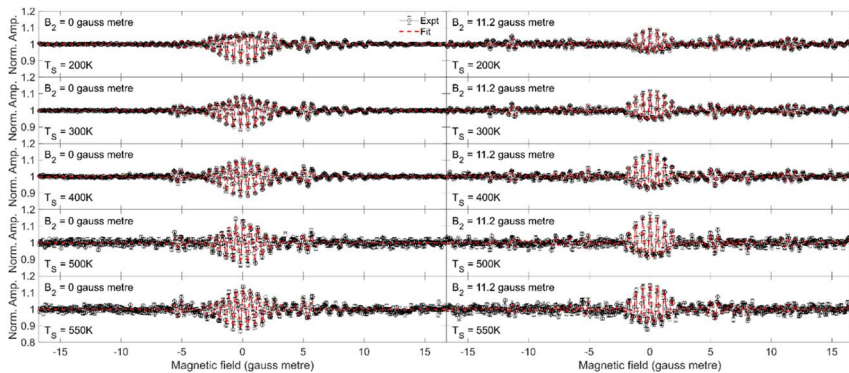
Fig. 5 Fits (red dashed line) to the experimental oscillation curves (black) measured for \text{H}_2 scattering from a Cu(511) surface at a temperature of 200 K (first row), 300 K (second row), 400 K (third row), 500 K (fourth row) and 550 K (fifth row) for B_2 = 0 gauss metre (left column) and B_2 = 11.2 gauss metre (right column).
