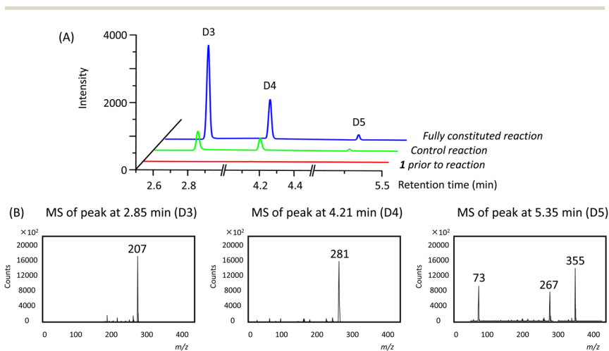
Fig. 4 Gas chromatograms (A) and mass spectra (B) of the reaction mixtures for substrate 1. The fragmentation patterns of D3, D4 and D5 are consistent with the electron ionisation fragmentation patterns observed for authentic standards.
