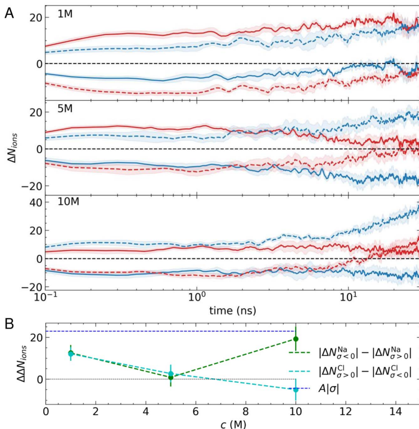
Fig. 2 (A) Changes to the mean number of ions ( \Delta N_{\text{ions}} ) in the EDL (defined as a 2.5 nm region adjacent to the carbon basal surface) when a surface charge is switched on with \sigma = \pm 0.77 \text{ e nm}^{-2} . Solid and dashed lines pertain to positively and negatively charged surfaces, and the blue and red colours indicate cations and anions, respectively. The data are averages from five independent simulations with the uncertainties calculated as the standard error of the mean in the data, as shown by the shaded regions. (B) A summary of the data in panel A, where the green and cyan points provide the differences between \Delta N_{\text{Na}} and \Delta N_{\text{Cl}} at the counter and co-electrode in the EDL. Dashed lines provide a linear interpolation between the data as a guide, while the blue dashed line provides the magnitude of the surface charge in units of e .
